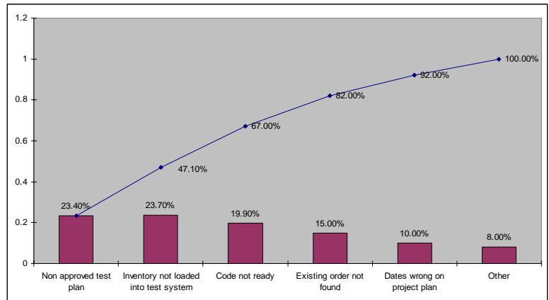
Figure 1. Pareto Chart
